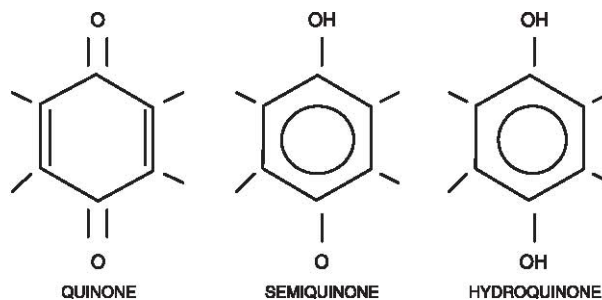
Figure 2 Core structure of idebenone demonstrating quinone, semiquinone, and hydroquinone redox forms.
